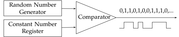
Fig. 1: Stochastic Number Generator.
